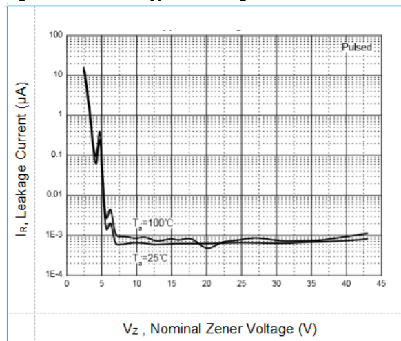
Fig6. BZX584C27V Typical Leakage Current
