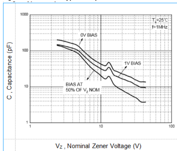
Fig5. BZX584C27V Typical Capacitance
