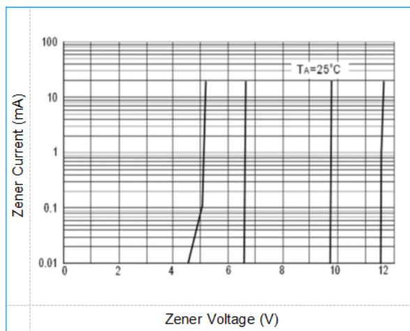
Fig2. BZX584C27V Zener Breakdown Characteristics
