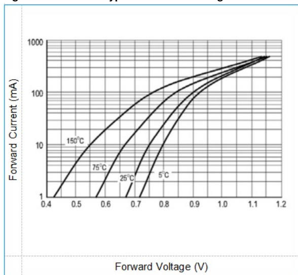
Fig3. BZX584C27V Typical Forward Voltage
