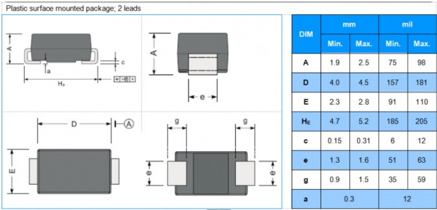
DO-214AC/SMA Package 1SMA4740A Outline & Dimensions:
