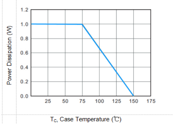
Zener Diode 1SMA4740A Curves: Fig. 1. 1SMA4740A Max. Continuous Power Derating
