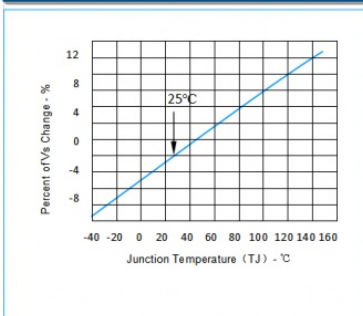
Fig.3: Normalized V_S change vs. junction temperature
