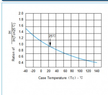
Fig.4: Normalized DC holding current vs. case temperature
